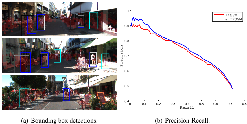
Fig. 7 Pedestrian detection on a high dynamic sequence. (a) Bounding box for ground truth (white), IKSVM [17] (blue and cyan) and weighted IKSVM with the evidence for the objects class inside the box (blue). The objects class is highlighted in red. (b) The precision-recall curve for this sequence with the IKSVM alone and weighted IKSVM by our objectness evidence.
