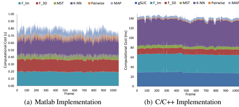
Fig. 8 Computational timing performance for a sequence in downtown with our recursive inference approach, see Fig. 5. We show the corresponding cost for image features ( F_{Im} ), 3D features ( F_{3D} ), MST, unary term (K-NN), pairwise term (Pairwise), and MAP assignment.
