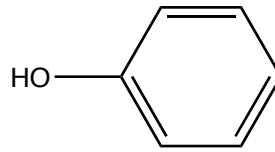
Phenol
