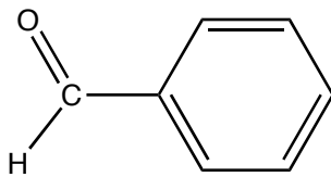
Benzaldehyd
