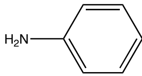
Anillin
