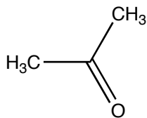
Keton Aceton
