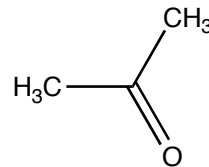
Aceton
