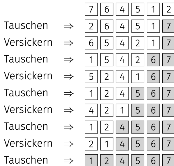
Abbildung 5.6: Heapsort
