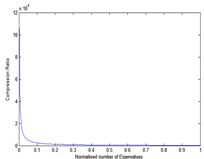
Fig. 11 Compression Ratio vs Normalized number of Eigen values
